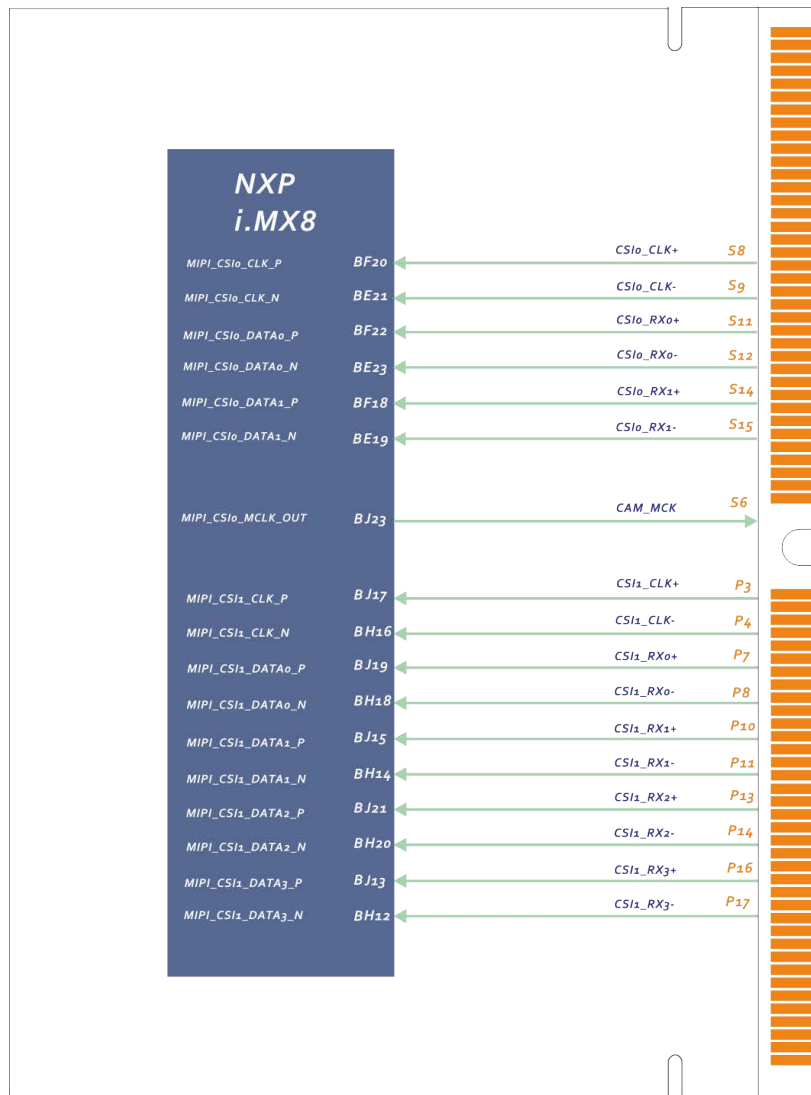
Figure 10 MIPI/Serial Camera Interface Block Diagram
