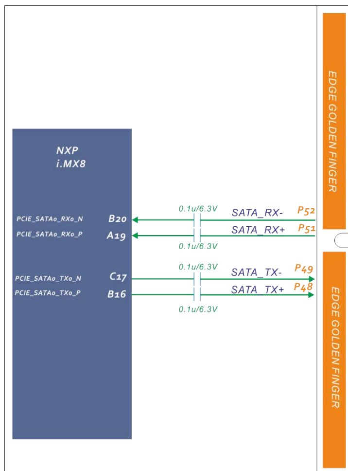
Figure 9 SATA Block Diagram
